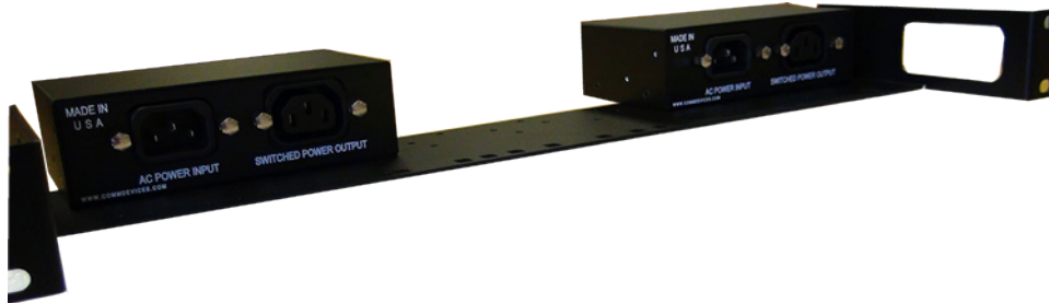
PCM BKT 801 Rack Mount 2 PCM605 devices
